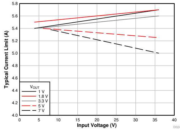
Figure 37. Current Limit Threshold
