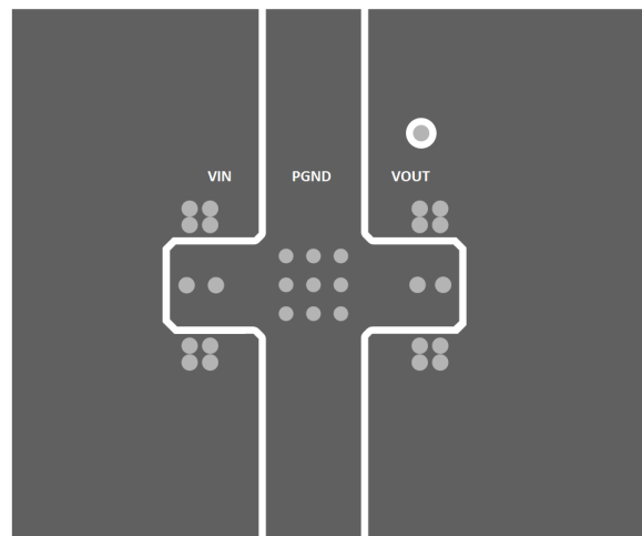
Figure 45. Typical Layer-2 Layout
