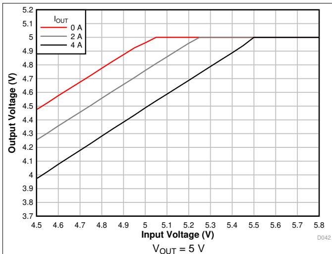
Figure 33. Voltage Dropout
