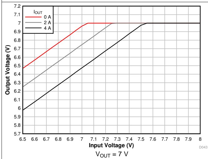
Figure 35. Voltage Dropout
