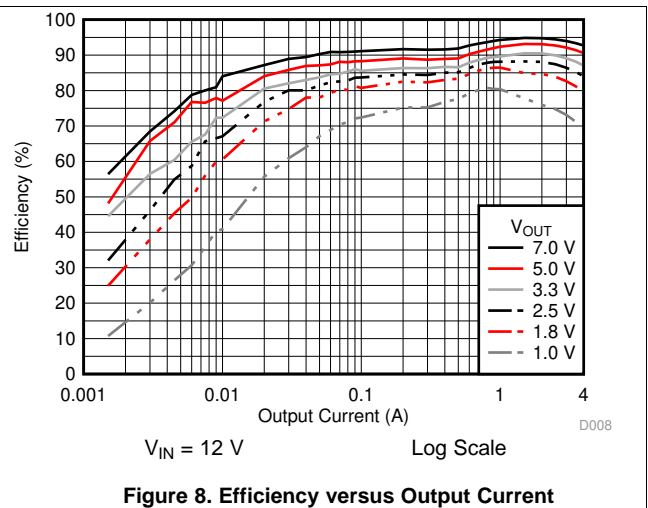
Figure 8. Efficiency versus Output Current
