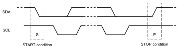
Figure 3 START and STOP conditions
