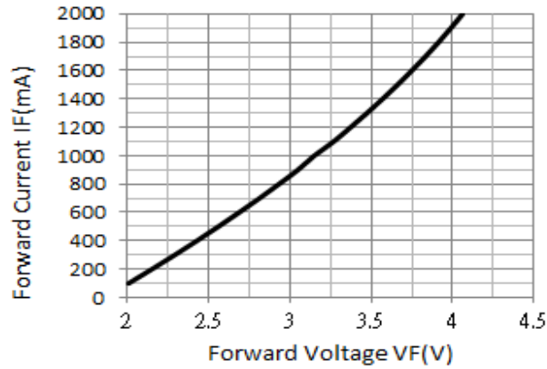
Fig 4. Forward Current
