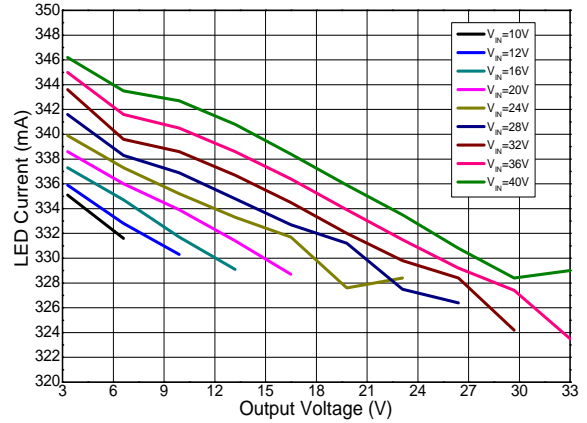
LED Current vs. Output Voltage ( R_{SET} = 0.3\Omega , L = 100\mu\text{H} )
