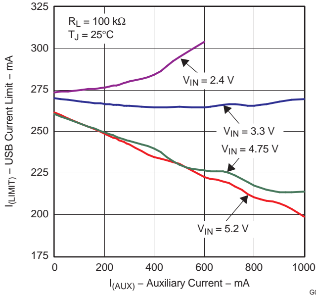
Figure 16. USB Current-Limit Threshold vs I_{AUX} , R_{ILIM} = 100\text{ k}\Omega , T_A = 25^\circ\text{C}
