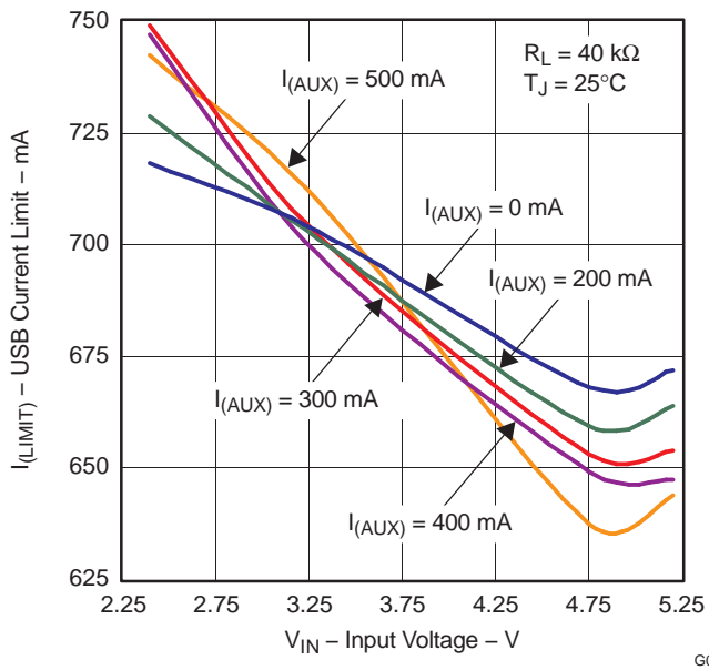
Figure 18. USB Current-Limit Threshold vs V_{IN} , R_{ILIM} = 40\text{ k}\Omega , T_A = 25^\circ\text{C}
