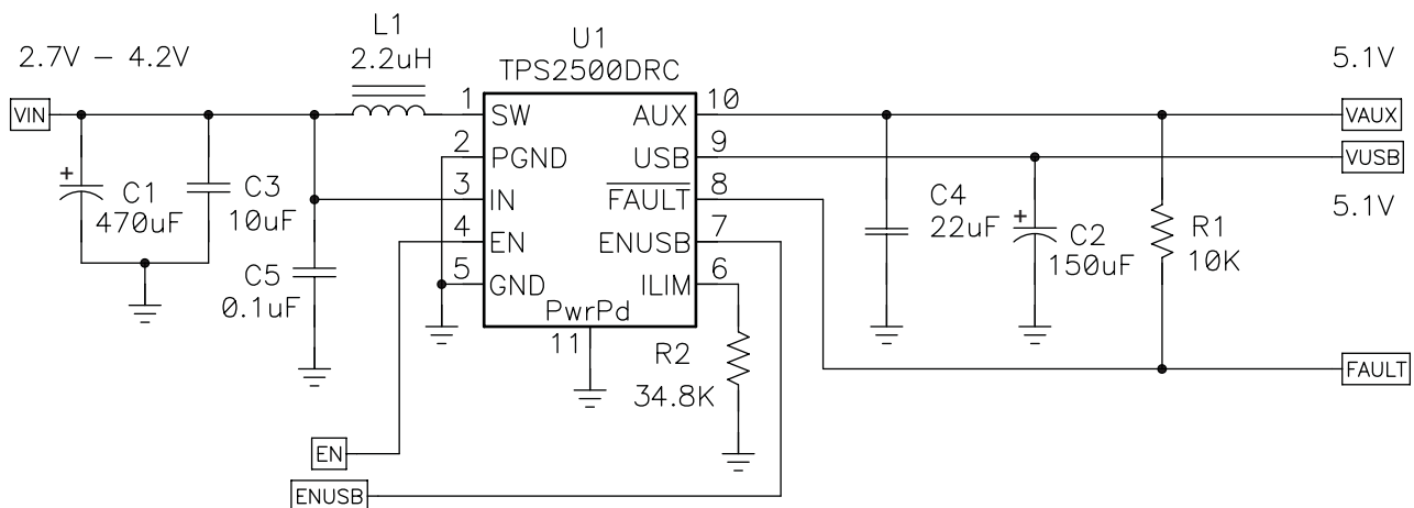
Figure 22. Reference Schematic
