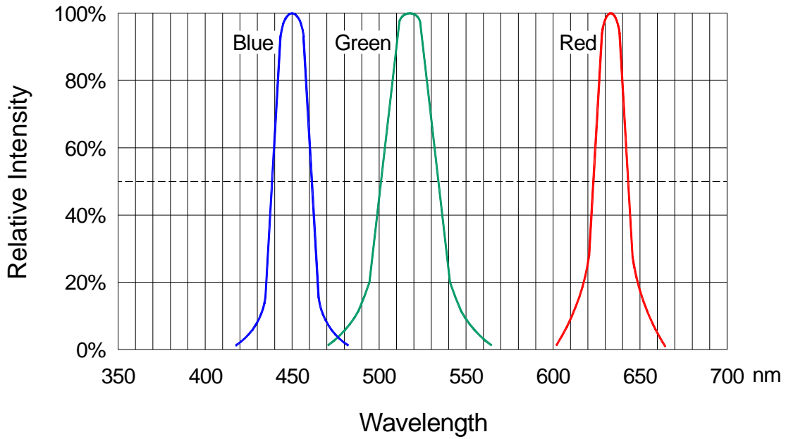
Fig.1 Relative Intensity vs Dominant Wavelength
