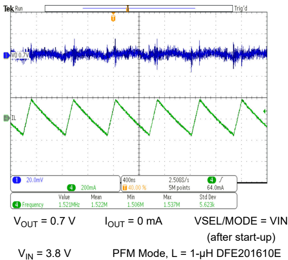
图 9-28. TPS62806 Typical Forced PWM Mode Operation (1.5 MHz)
