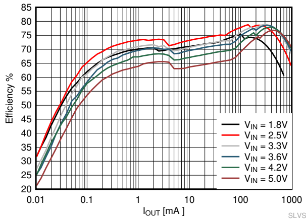
TPS62800 R_{VSEL} = 10\text{ k}\Omega to GND
