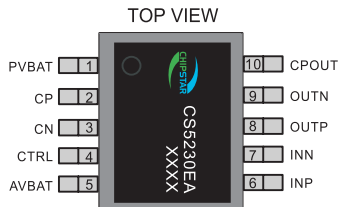
CS5230EA(ESOP10 PACKAGE)
