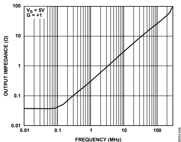
Figure 31. Closed-Loop Output Impedance vs. Frequency, Part Enabled
