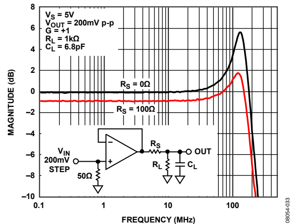
Figure 57. Closed-Loop Frequency Response with Snub Resistor, C_L = 6.8\text{ pF}
