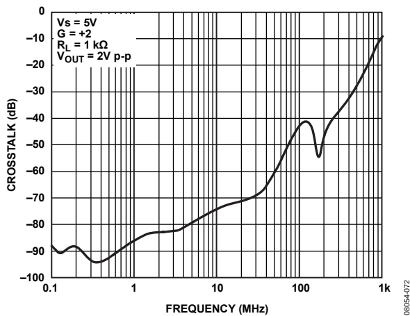
Figure 45. All-Hostile Crosstalk (Output-to-Output) vs. Frequency
