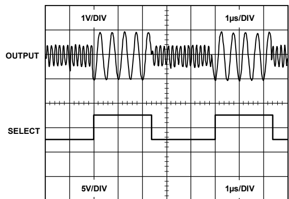
Figure 65. ADA4891-3 Mux Output
