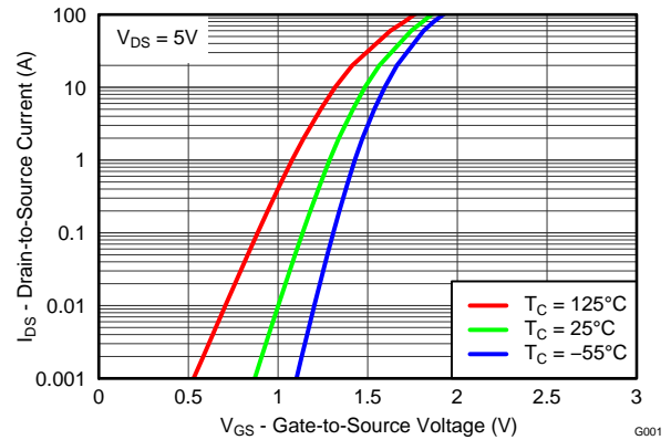
Figure 13. Sync MOSFET Transfer
