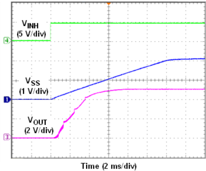
Figure 34. Inhibit Turn-On
