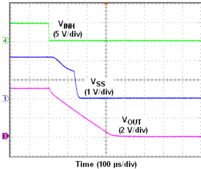
Figure 33. Inhibit Turn-Off
