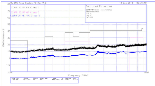
图 8-33. Radiated EMI Log-periodic Antenna (Vertical)
