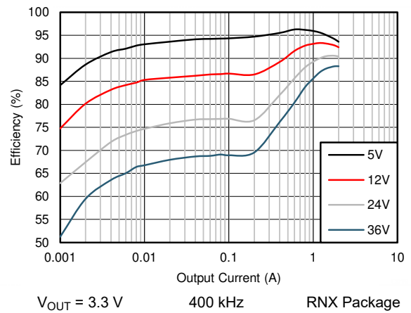
图 8-12. Efficiency
