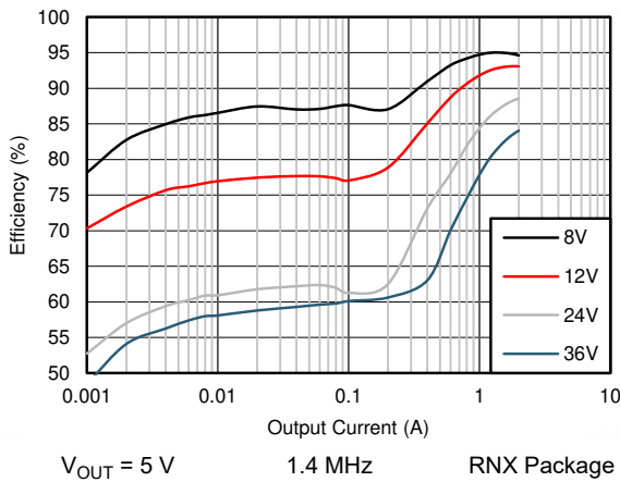
图 8-13. Efficiency
