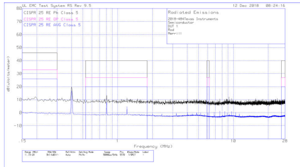
图 8-34. Radiated EMI Rod Antenna
