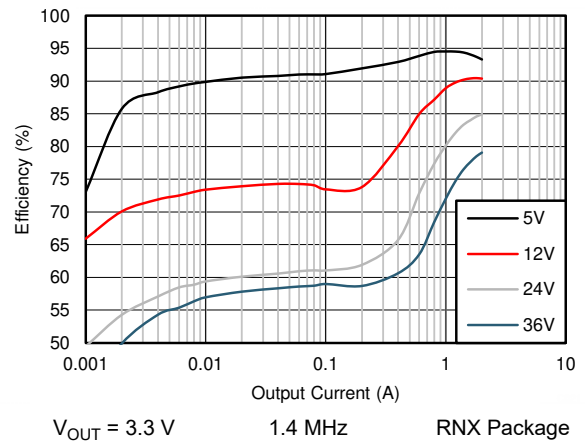
图 8-14. Efficiency
