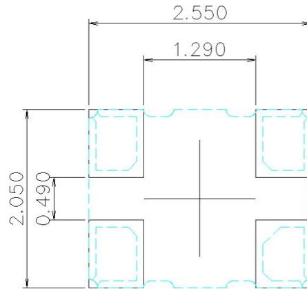
Reference Land Pattern
