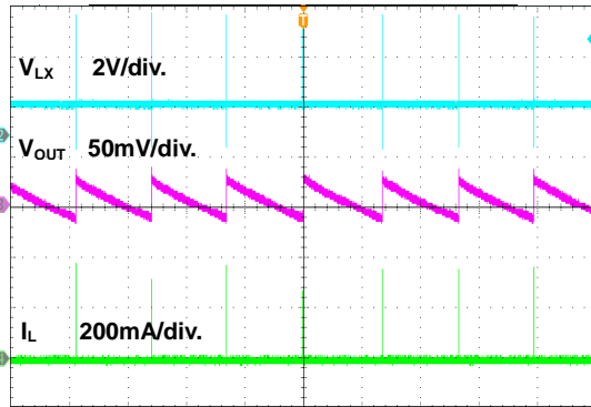
Figure 16. Steady State Waveform
