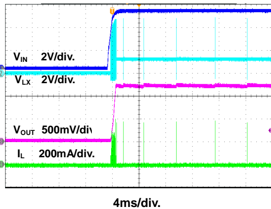
Figure 8. Power On through VIN Waveform
