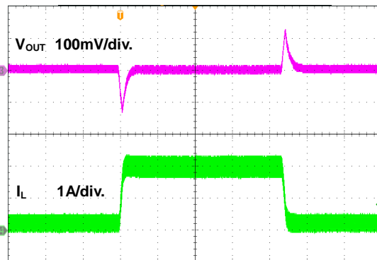
Figure 18. Load Transient Waveform
