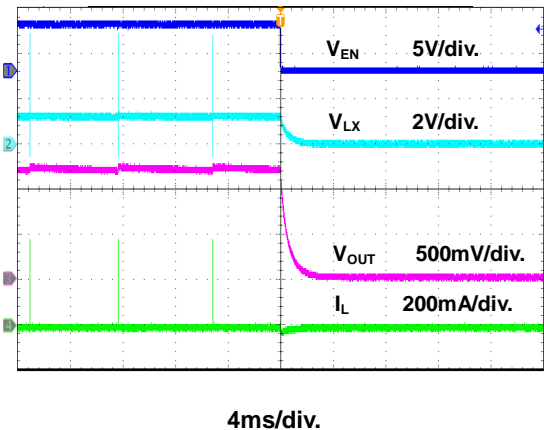
Figure 14. Power Off through EN Waveform
