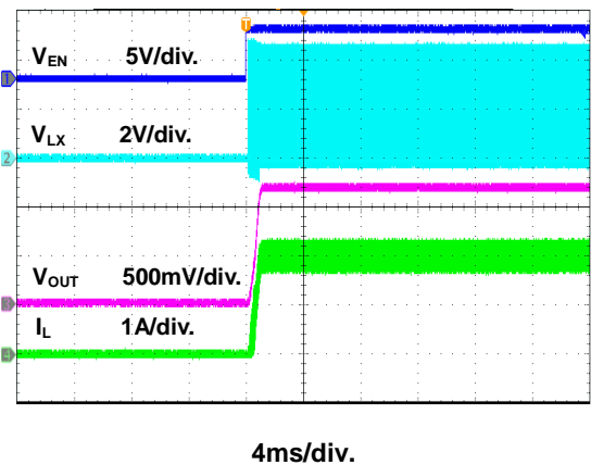
Figure 13. Power On through EN Waveform
