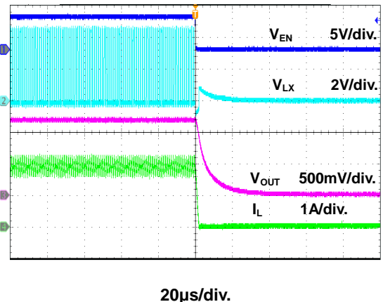
Figure 15. Power Off through EN Waveform
