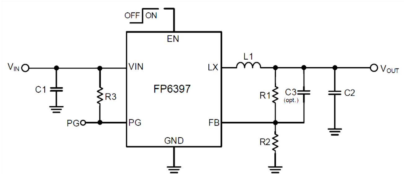
Figure 2. Schematic Diagram
