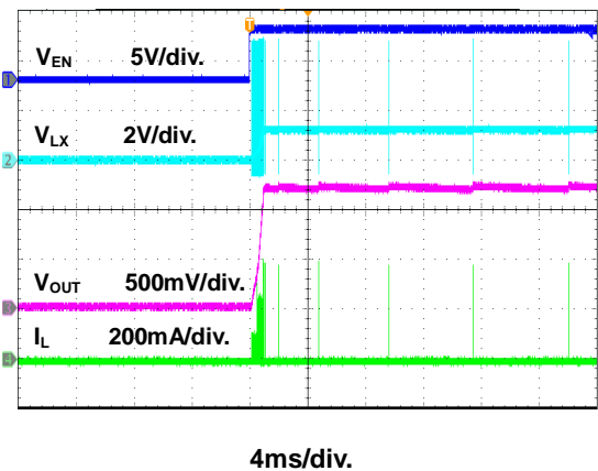
Figure 12. Power On through EN Waveform
