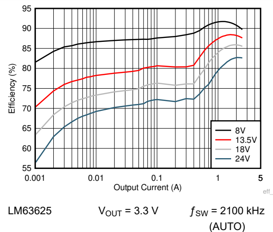
Figure 9-13. Efficiency
