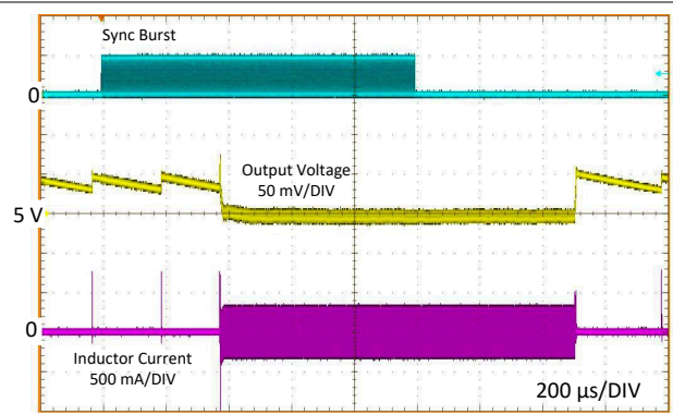
Figure 8-11. Typical Transition from Sync Mode to FPWM Mode V_{IN} = 12\text{ V} , V_{OUT} = 5\text{ V} , I_{OUT} = 1\text{ mA}
