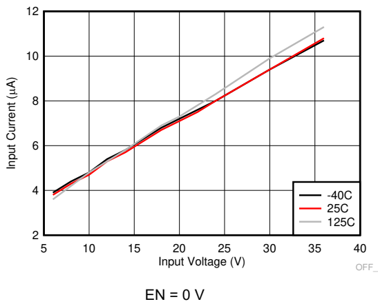
Figure 7-1. Input Supply Current in Shutdown Mode
