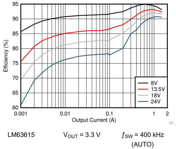
Figure 9-14. Efficiency
