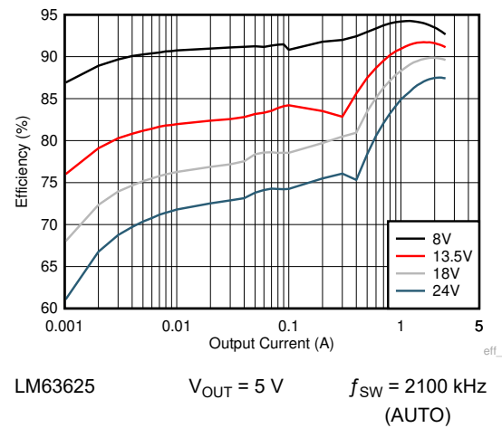
Figure 9-9. Efficiency
