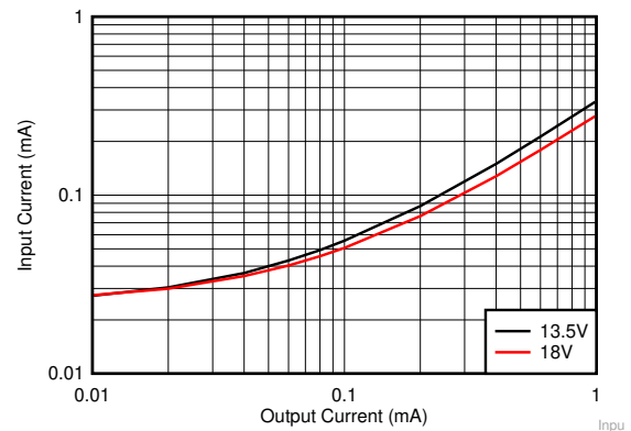
LM63615 V_{OUT} = 3.3\text{ V} f_{SW} = 2100\text{ kHz} (AUTO)
