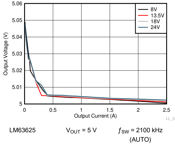
Figure 9-16. Line and Load Regulation
