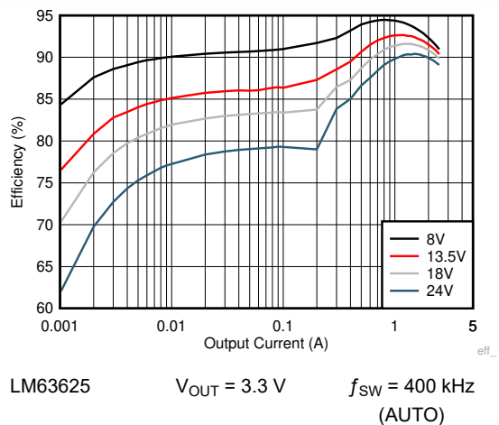
Figure 9-12. Efficiency
