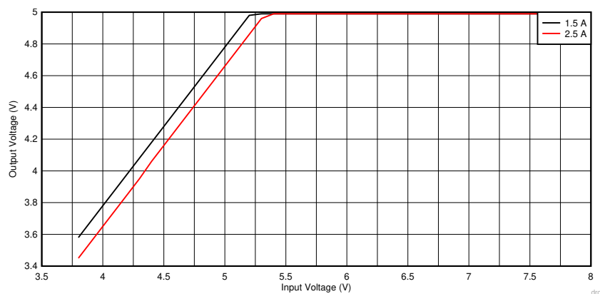
Figure 8-12. Overall Dropout Characteristic V_{OUT} = 5\text{ V}
