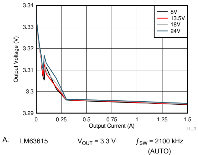
Figure 9-19. Line and Load Regulation
