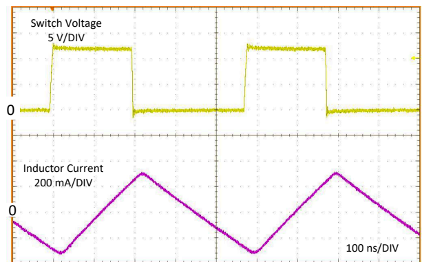
Figure 8-7. Typical PWM Switching Waveforms Without Spread Spectrum V_{IN} = 12\text{ V} , V_{OUT} = 5\text{ V} , I_{OUT} = 2.5\text{ A} , f_{SW} = 2100\text{ kHz}
