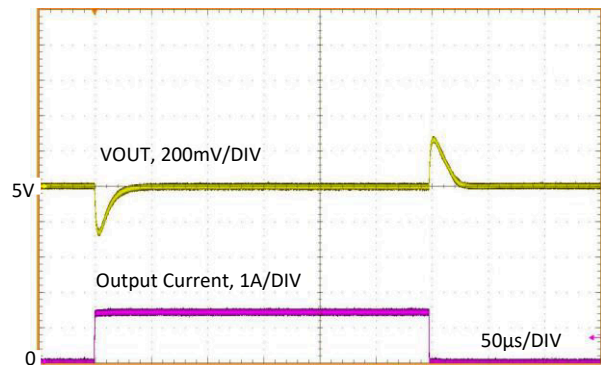
Figure 9-27. Load Transient
