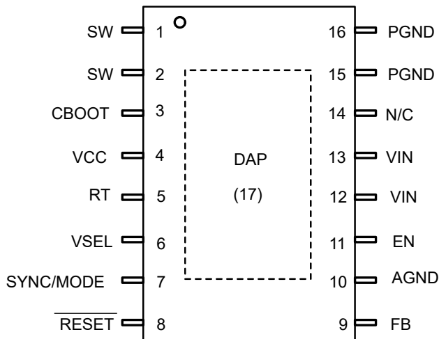
Figure 6-1. 16-Pin HTSSOP With PowerPAD PWP Package (Top View)
