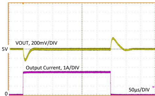
Figure 9-26. Load Transient
