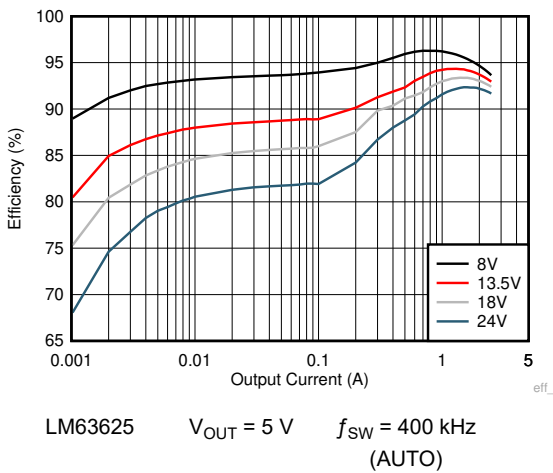
Figure 9-8. Efficiency
