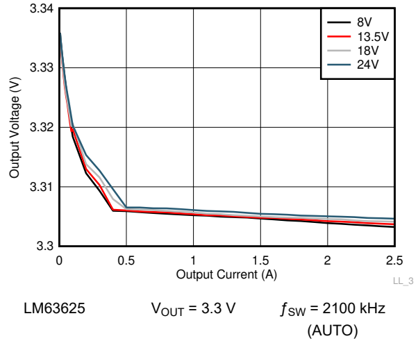
Figure 9-17. Line and Load Regulation
