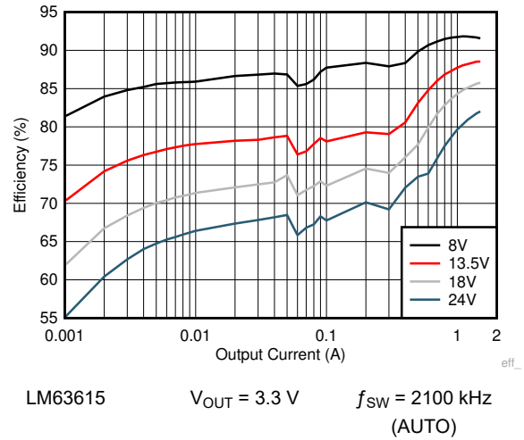
Figure 9-15. Efficiency
