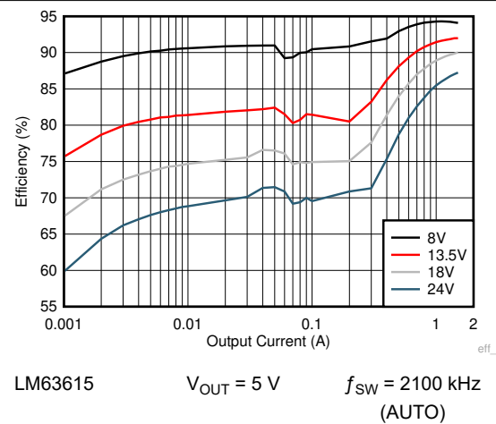
Figure 9-11. Efficiency
