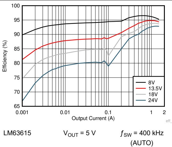
Figure 9-10. Efficiency
