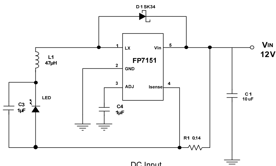
DC Input LED Application Circuit
