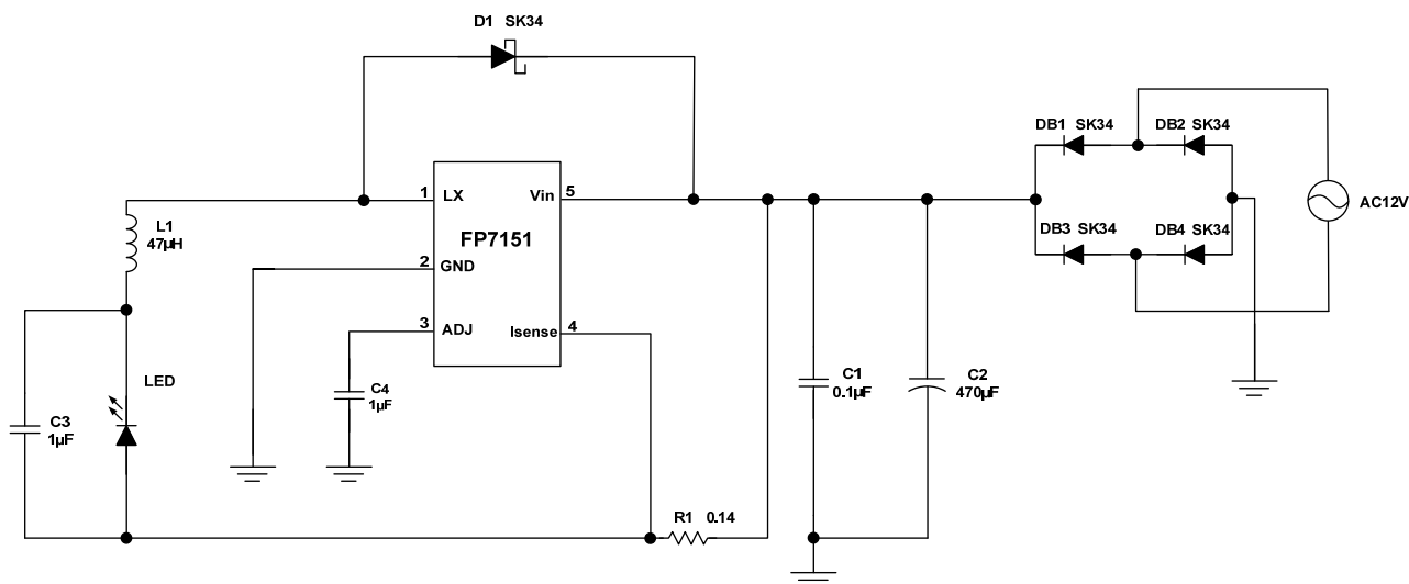
AC Input LED Application Circuit
