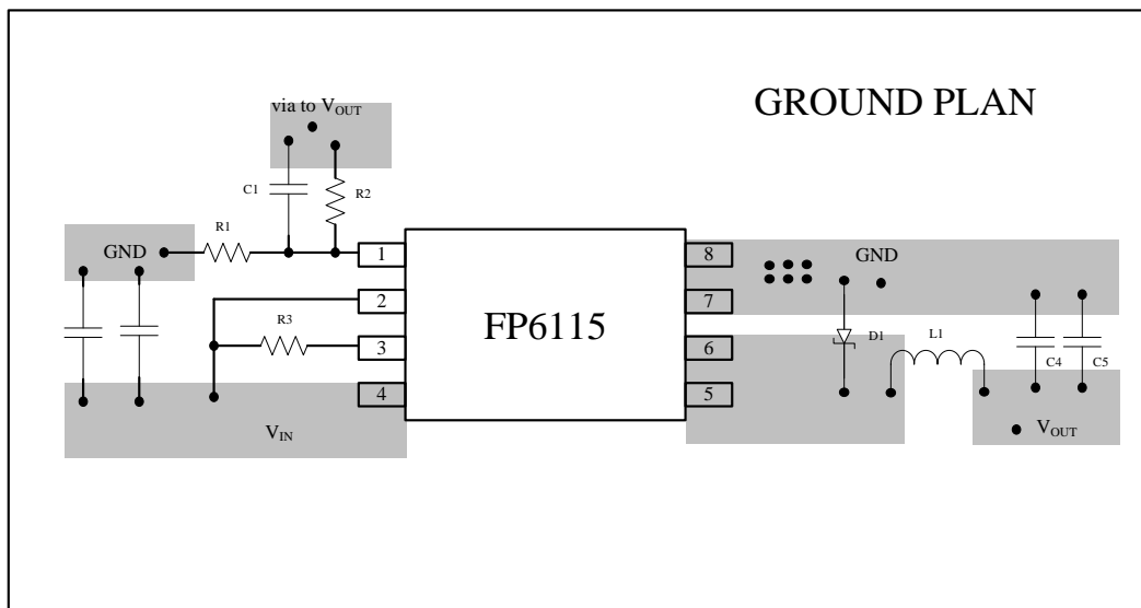
Suggested Layout
