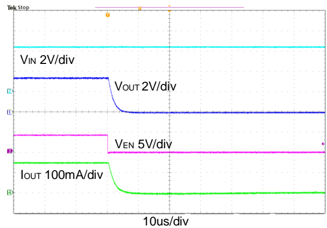
Figure 7. EN Turn OFF Waveform
