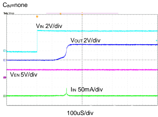
Figure 5. V_{IN} Turn On Inrush Current
