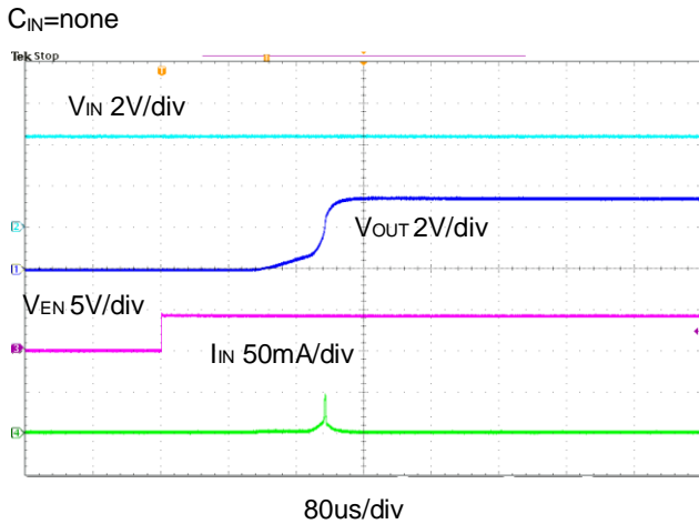
Figure 4. EN Turn On Inrush Current
