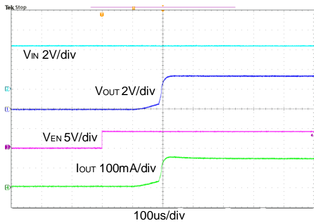
Figure 6. EN Turn On Waveform
