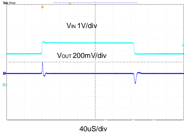
Figure 11. Line Transient Response
