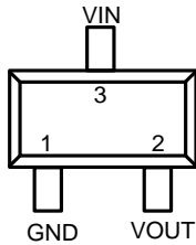
Figure 1. Pin Assignment of FP6182
