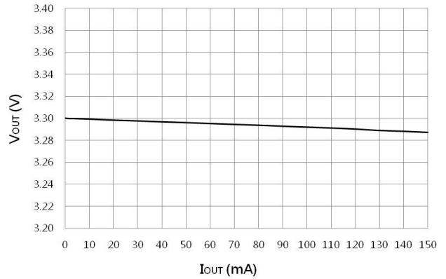
Figure 13. Output Voltage vs. Output Current
