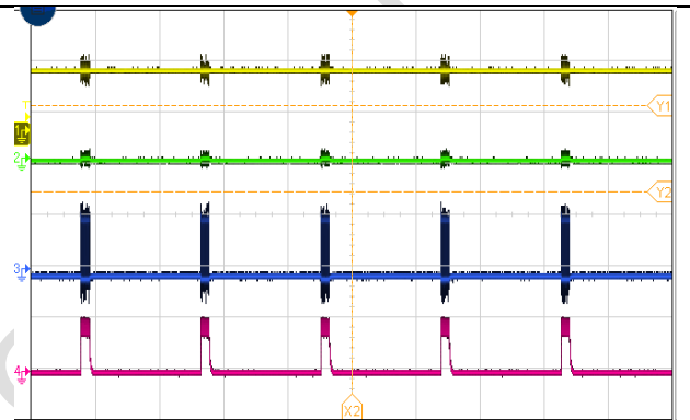
Fig.17 Steady State, Iout =0.6A
