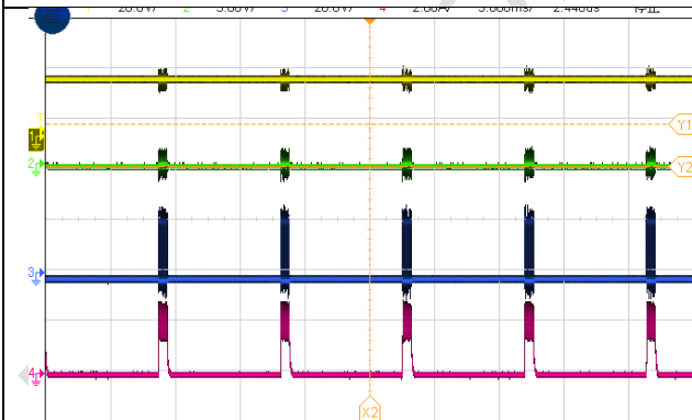
Fig.18 Steady State, Iout =0.6A
