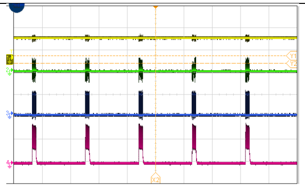
Fig.18 Short Circuit waveform
