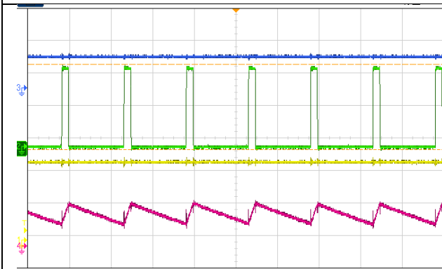
Fig.16 Steady State, Iout =0.6A
