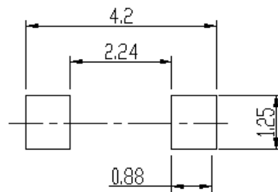
Soldering footprint
