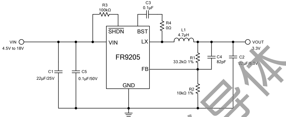
Figure 2. FR9205 Application Circuit
