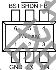
Figure 1. Pin Assignments of FR9205
