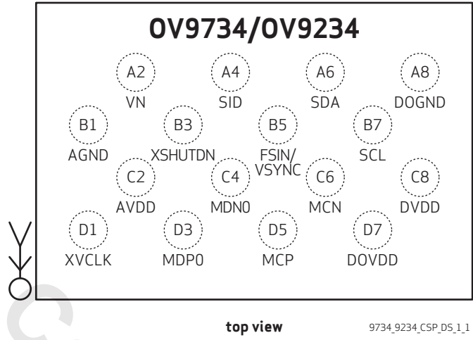
figure 1-1 pin diagram
