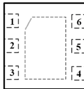
DFN2*2-6L
