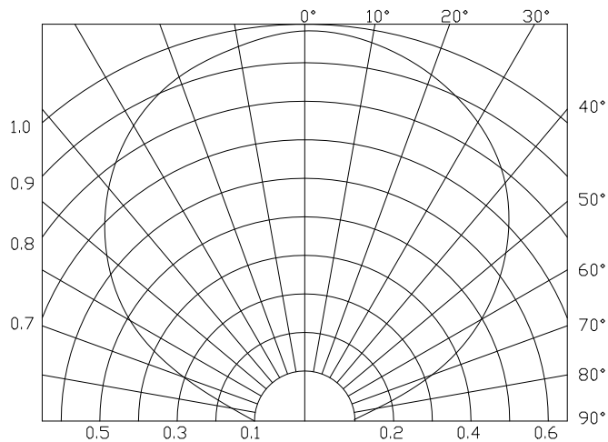
Radiation Diagram
