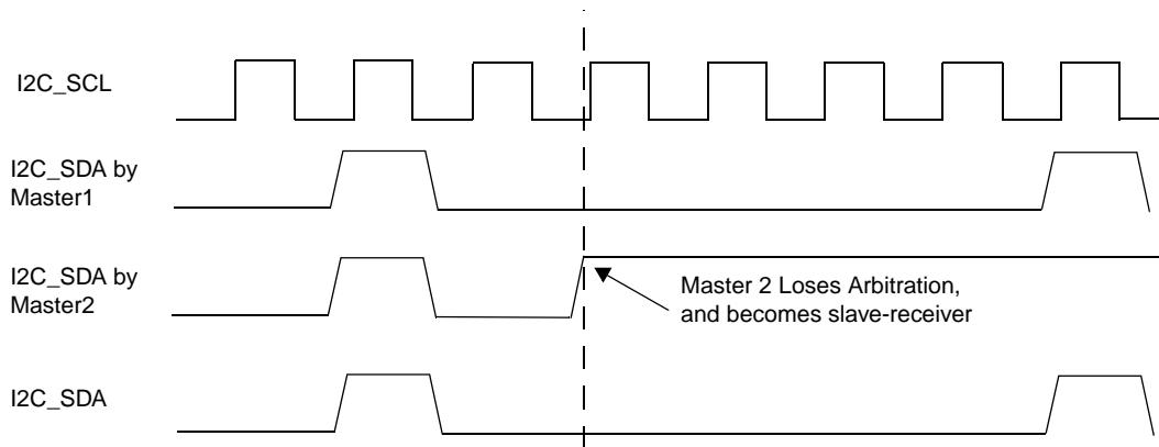
Figure 24-13. Arbitration Procedure
