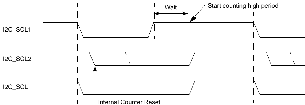
Figure 24-12. Clock Synchronization
