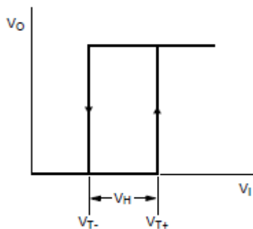
Figure 6. Transfer characteristic
