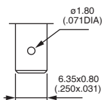
Normalized quick-connect 6.35x0.8
