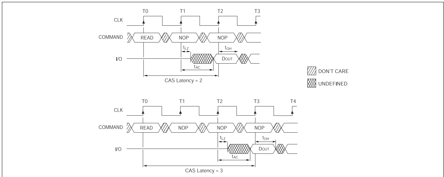
FIGURE 4 – CAS LATENCY
