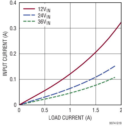
Input vs Load Current V_{OUT} = 1V
