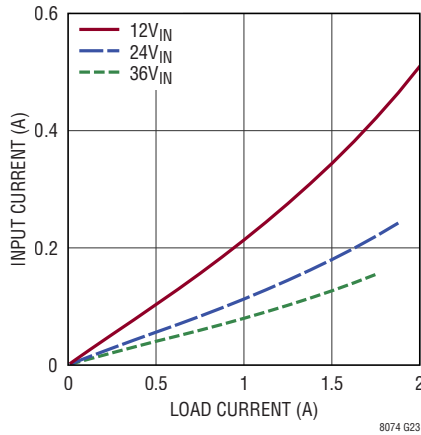
Input vs Load Current V_{OUT} = 2V
