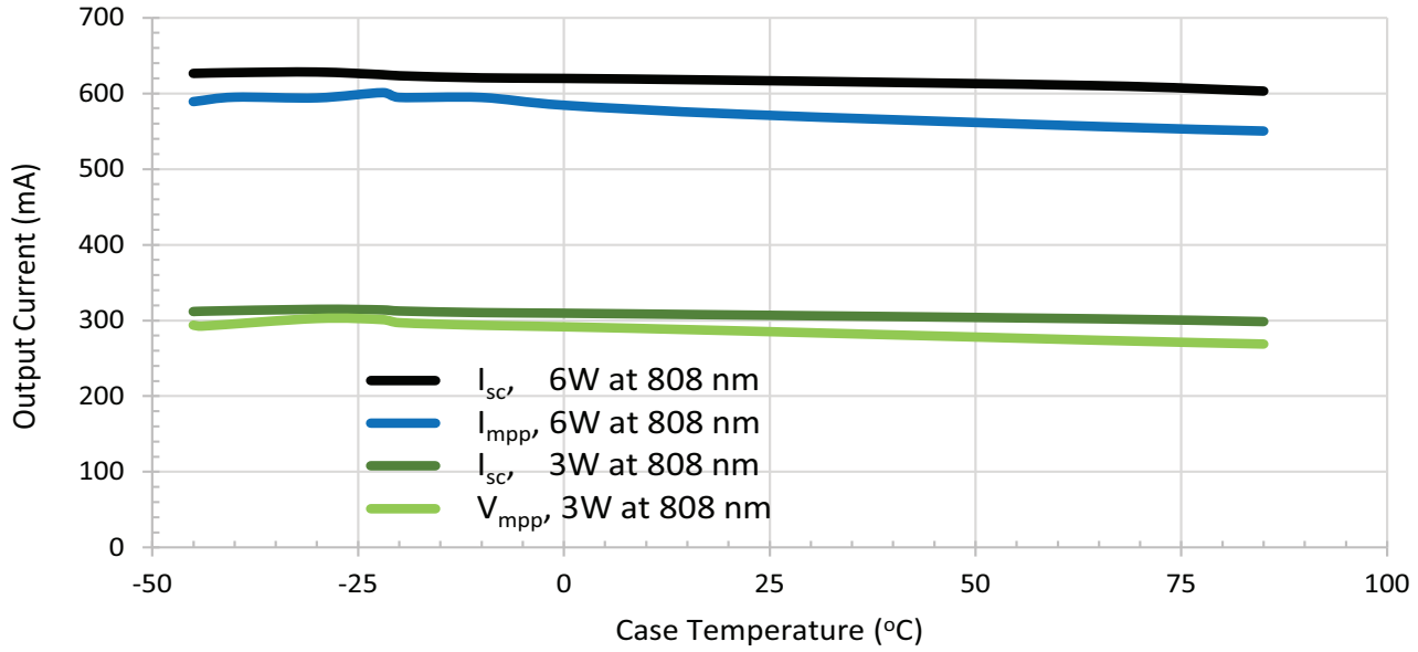
Figure 10: Typical Output Current ( I_{sc} & I_{mpp} ) vs. Case Temperature for the AFBR-POC306A1 at 808 nm
