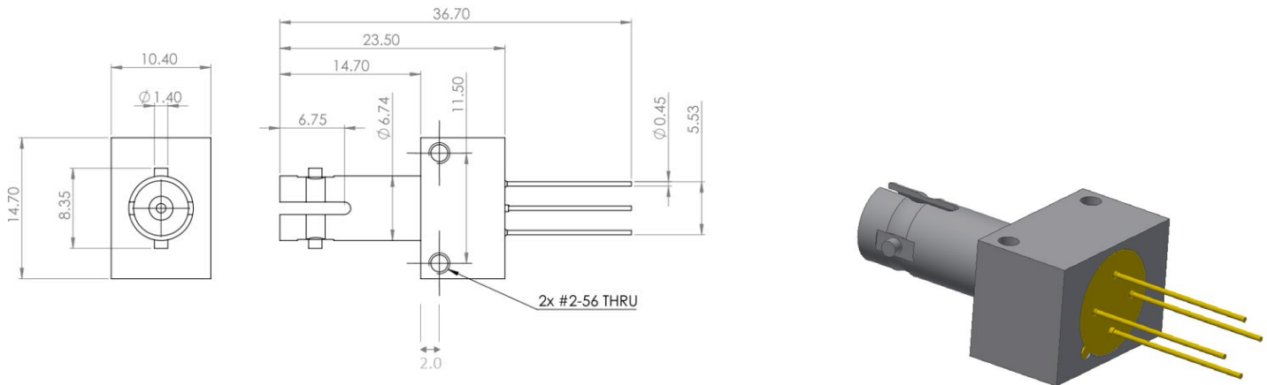
Figure 1: AFBR-POC3xxAx (4 Pins)
