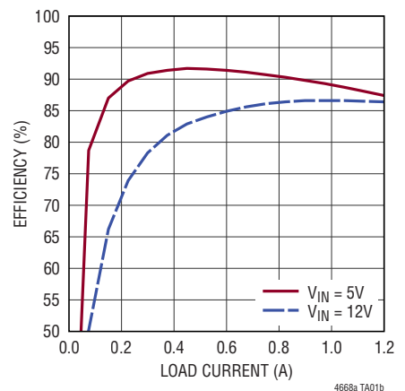
3.3V Output Efficiency (Each Channel)
