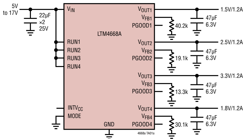
5V to 17V Input, Quad 1.5V, 1.8V, 2.5V, 3.3V Output DC/DC \mu Module Regulator
