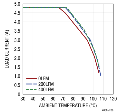
Figure 9. 12V to 1.8V Derating Curve, No Heat Sinking
