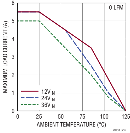
LTM8053 Derating, V OUT = 5V, BIAS = 5V, DC1934A Demo Board
