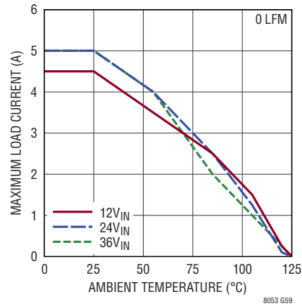
LTM8053 Derating, V OUT = -8V, BIAS Tied to LTM8053 GND, DC1934A Demo Board
