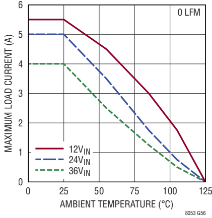
LTM8053 Derating, V OUT = 8V, BIAS = 5V, DC1934A Demo Board
