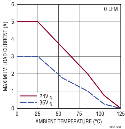
LTM8053 Derating, V OUT = -5V, BIAS Tied to LTM8053 GND, DC1934A Demo Board
