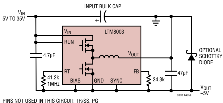
-5V OUT from 5V IN to 35V IN Positive to Negative Converter, BIAS tied to LTM8003 GND
