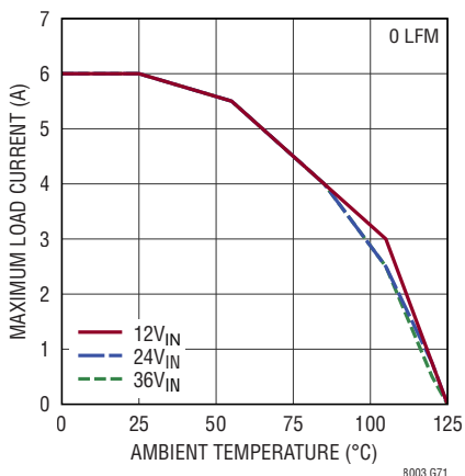
Derating, I-Grade, V_{OUT} = 0.97\text{V} , BIAS = 5V, DC2416A Demo Board
