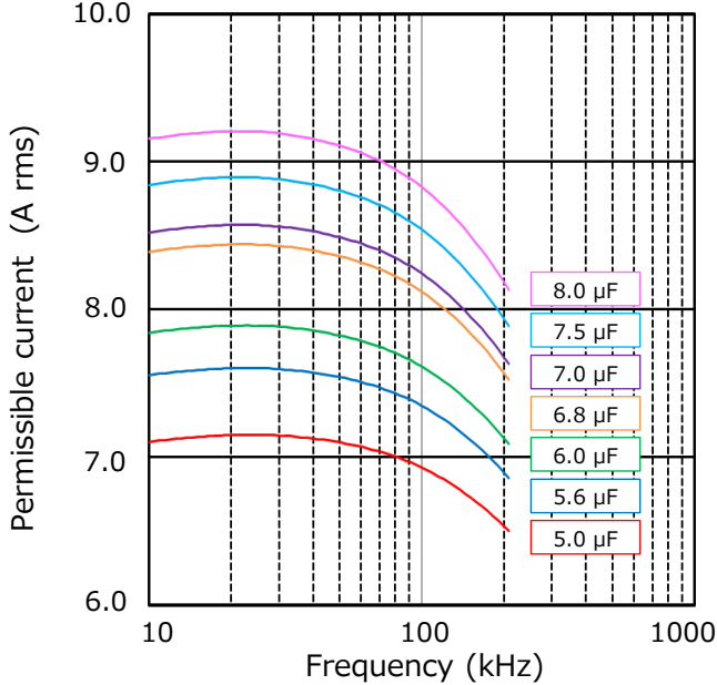
[ Permissible Current ]
