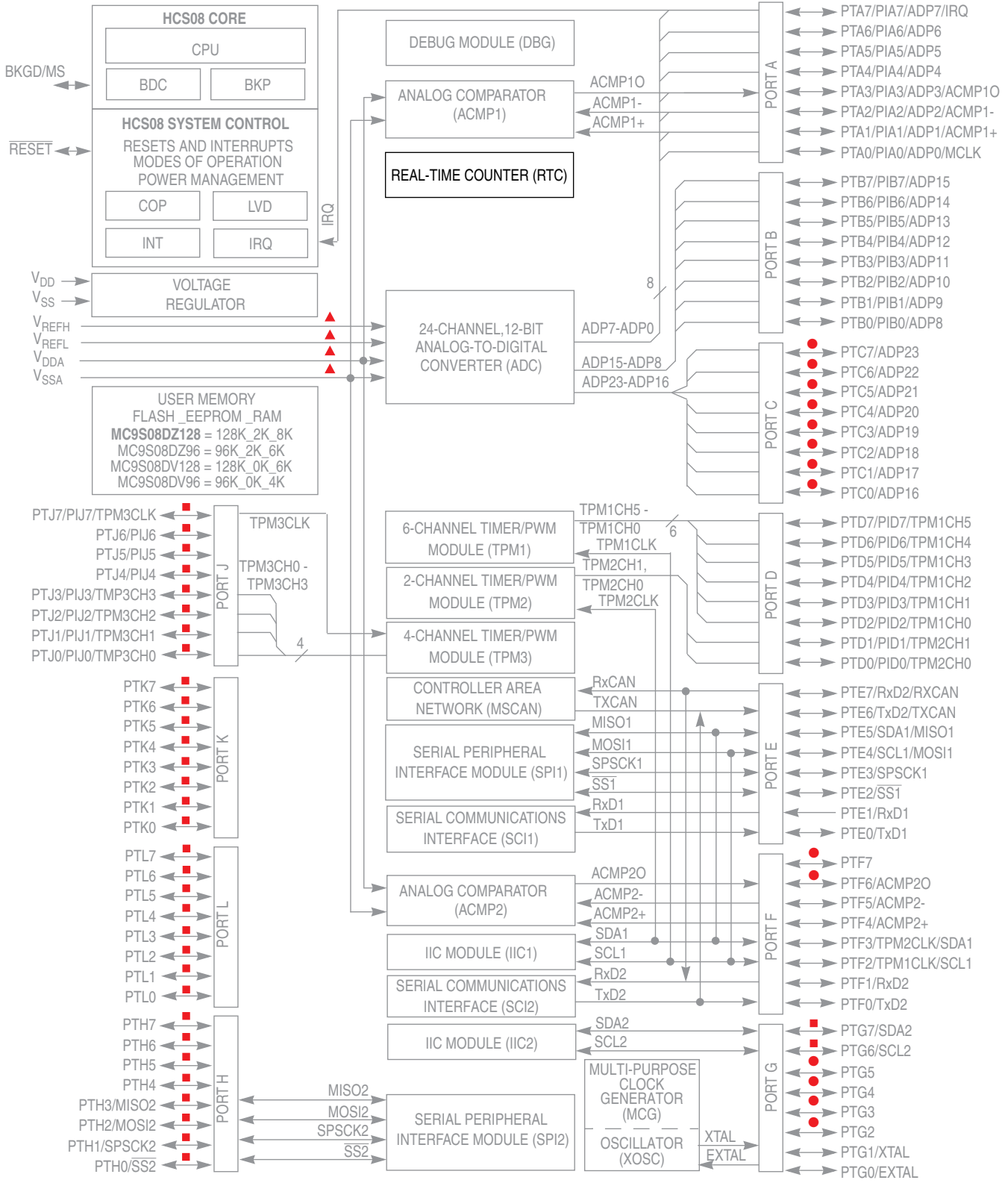
Figure 15-1. MC9S08DZ128 Block Diagram with RTC Highlighted
