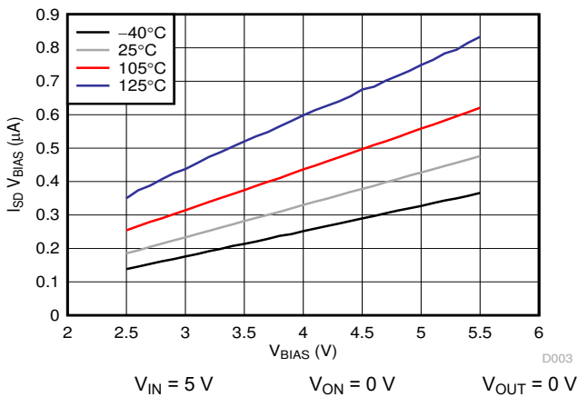
Figure 7-3. I SD V BIAS vs V BIAS
