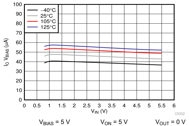
Figure 7-2. I Q V BIAS vs V IN
