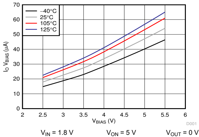
Figure 7-1. V BIAS Quiescent Current vs V BIAS
