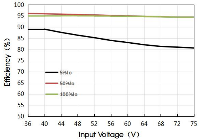
VCF4824QBO-400W(F/H)R3(-N) Efficiency VS Input Voltage
