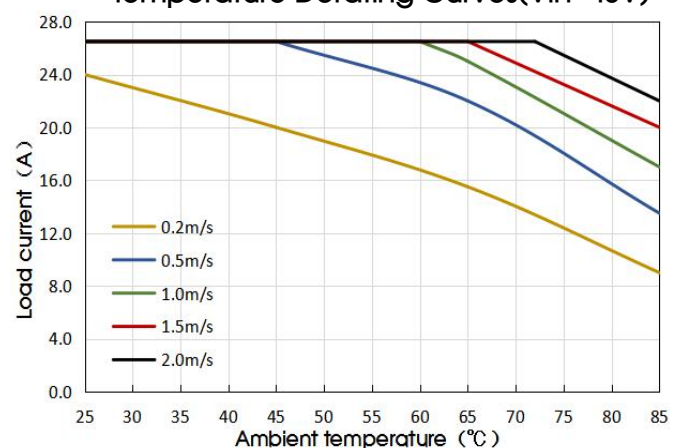
VCF4815QBO-400WHR3(-N) Temperature Derating Curves(Vin=48V)
