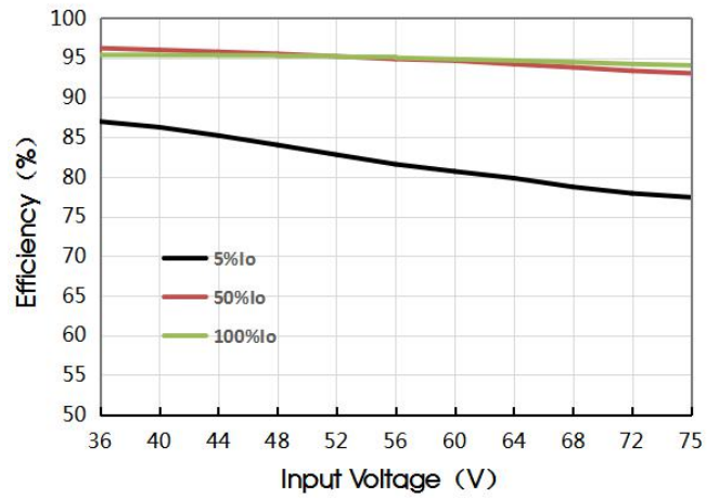
VCF4815QBO-400W(F/H)R3(-N) Efficiency VS Input Voltage
