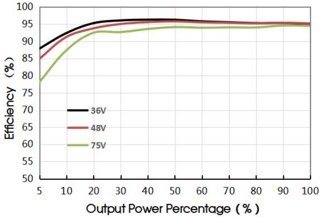
VCF4815QBO-400W(F/H)R3(-N) Efficiency VS Output Load
