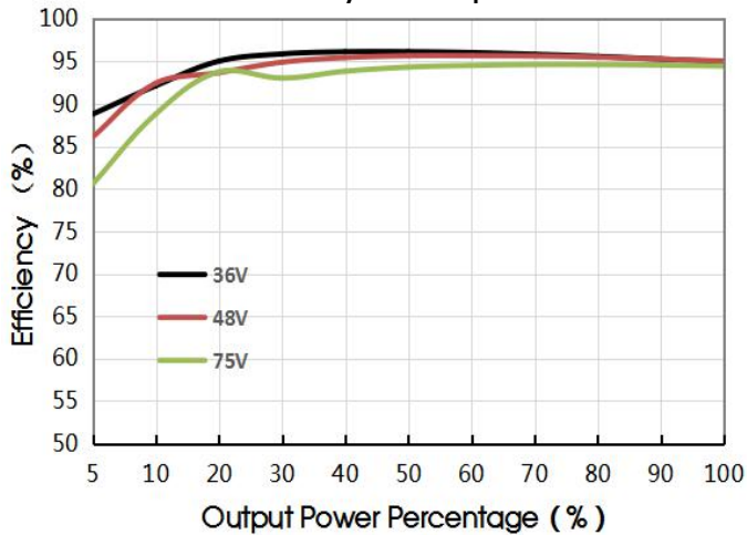
VCF4824QBO-400W(F/H)R3(-N) Efficiency VS Output Load
