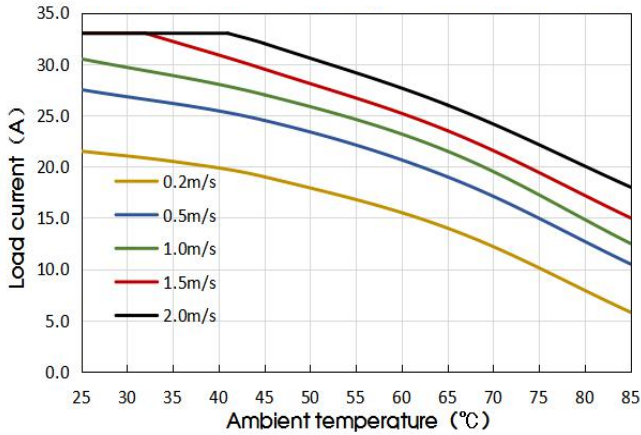
VCF4812QBO-400WR3(-N) Temperature Derating Curves(Vin=48V)
