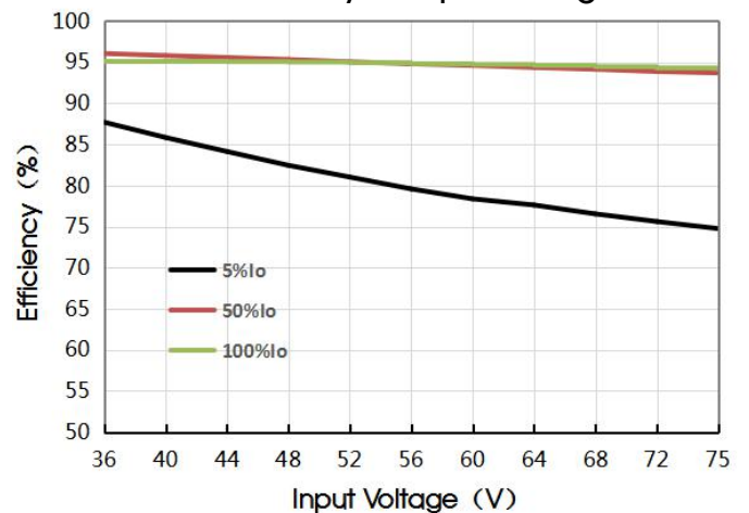
VCF4828QBO-400W(F/H)R3(-N) Efficiency VS Input Voltage
