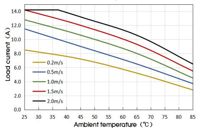
VCF4828QBO-400WR3(-N) Temperature Derating Curves(Vin=48V)
