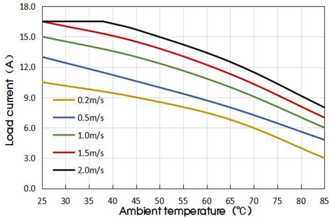
VCF4812QBO-400WHR3(-N) Temperature Derating Curves(Vin=48V)
