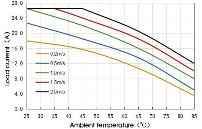
VCF4815QBO-400WR3(-N) Temperature Derating Curves(Vin=48V)
