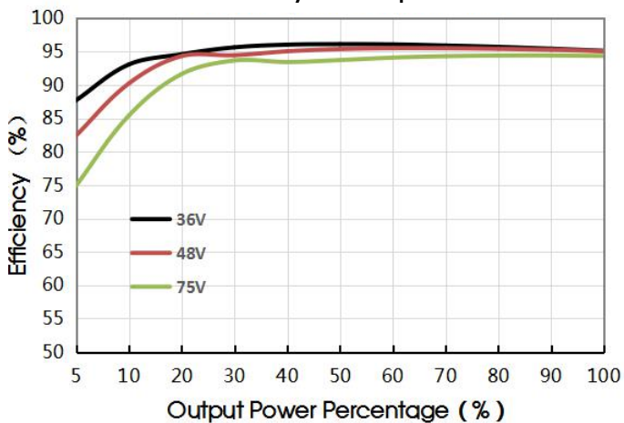
VCF4828QBO-400W(F/H)R3(-N) Efficiency VS Output Load
