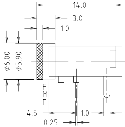
Model: Jack Socket Switched Part No. FC68133
