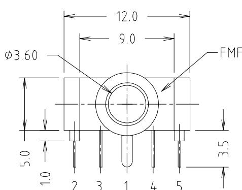
Model: Jack Socket Unswitched Part No. FC68131
