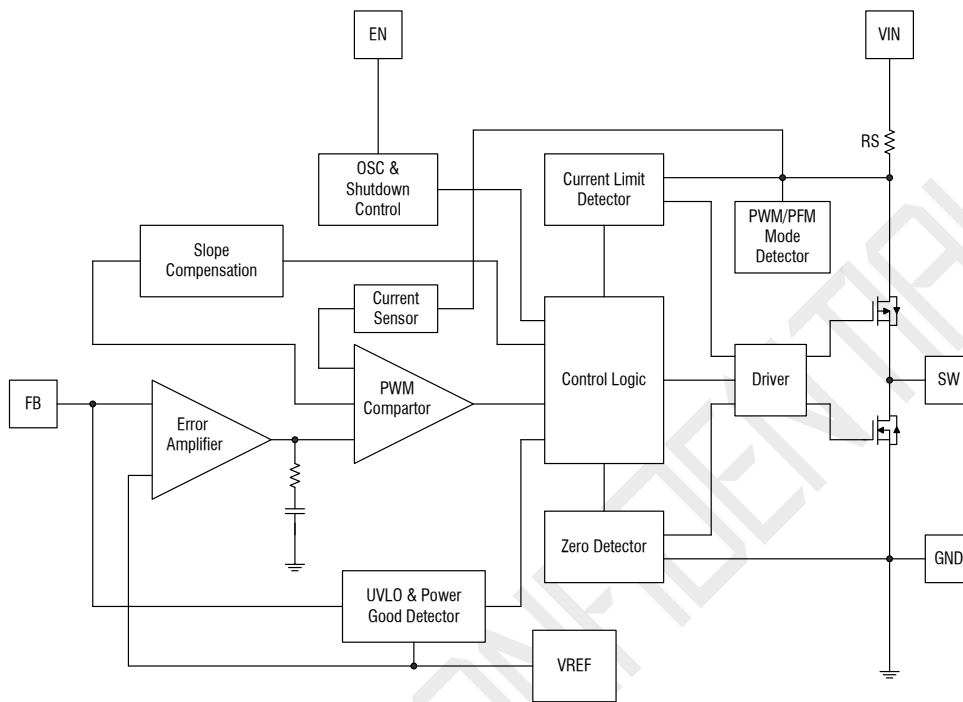
Figure 2. MT3428 Block Diagram
