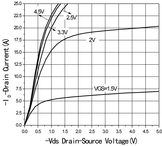
Fig1 Output Characteristics
