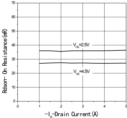
Fig3 R_{DS(on)} -Drain current
