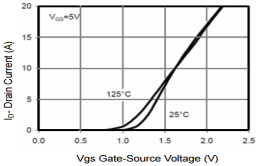
Figure 7 Transfer Characteristics
