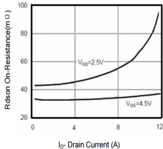
Figure 6 Drain-Source On-Resistance
