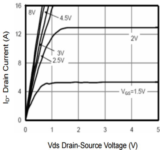
Figure 5 Output Characteristics
