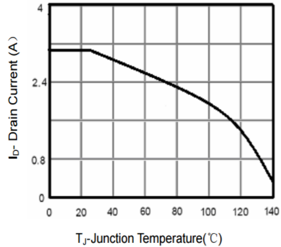
Figure 4 Drain Current
