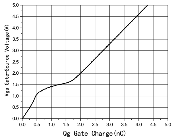
Fig6 Gate Charge
