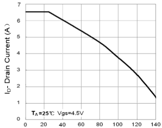
Figure 4 Drain Current
