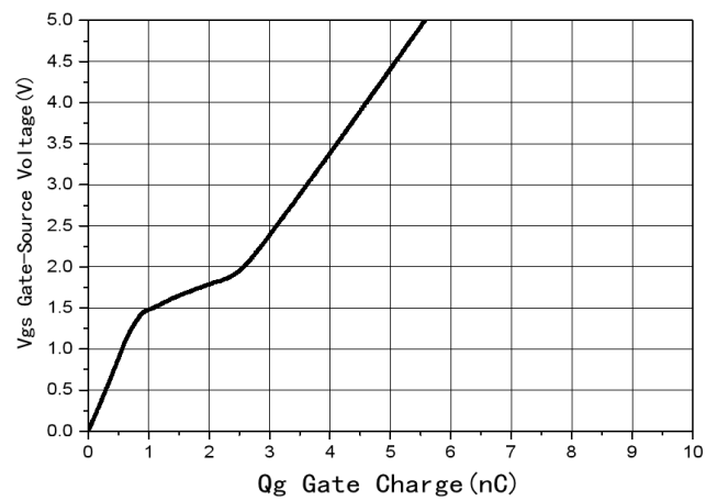
Fig6 Gate Charge
