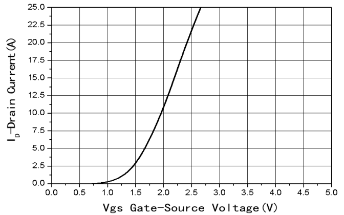
Fig2 Transfer Characteristics
