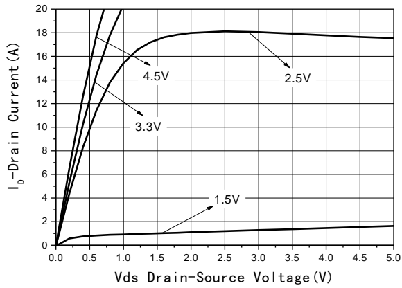
Fig1 Output Characteristics
