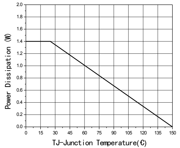
Fig4 Power De-rating
