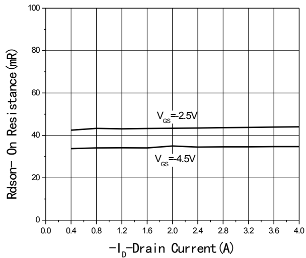
Fig3 Rds(on)-Drain current
