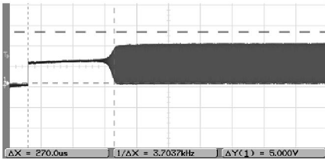
4MHz Ceramic
