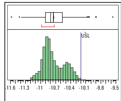
Return Loss at 12 GHz
