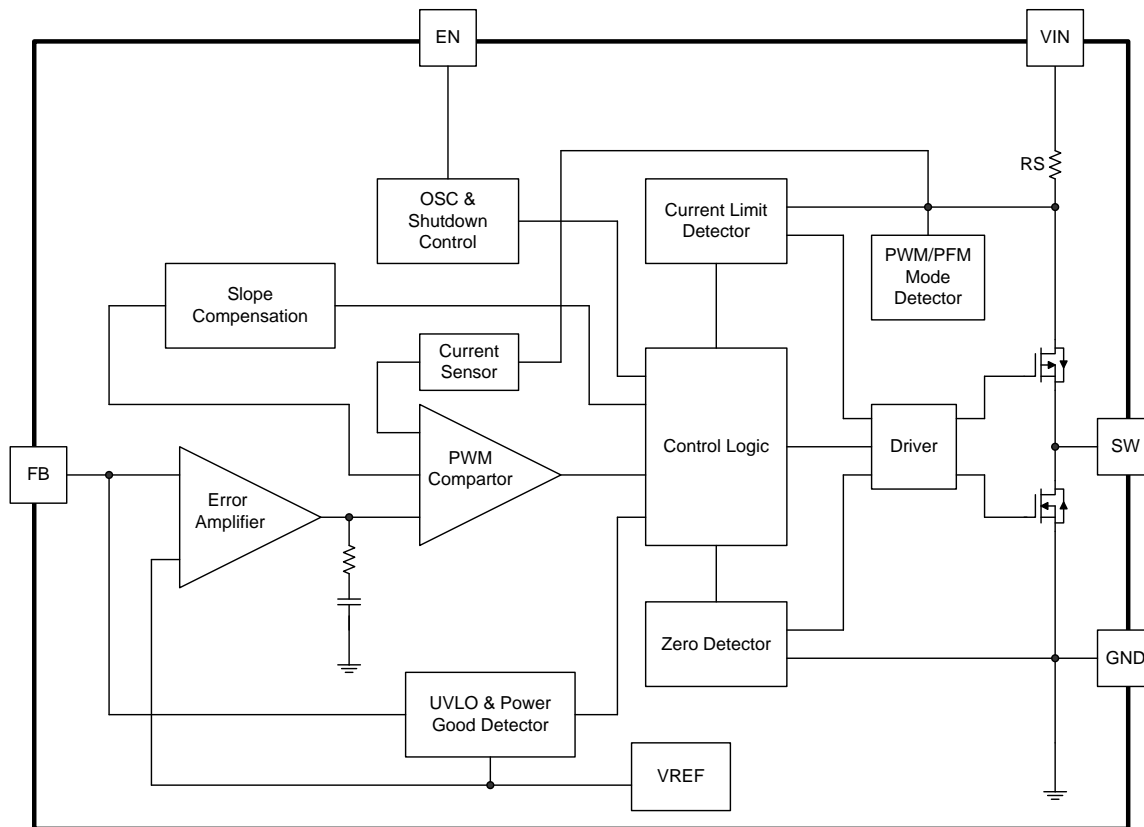
Block Diagram
