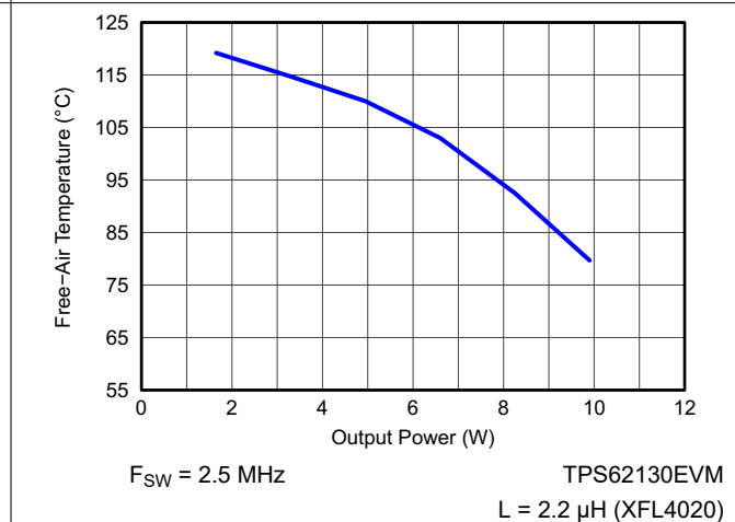
图 9-39. Maximum Ambient Temperature
